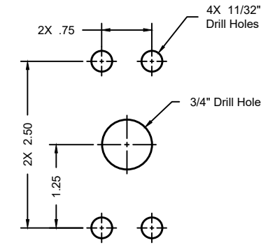
DRILL TEMPLATE
