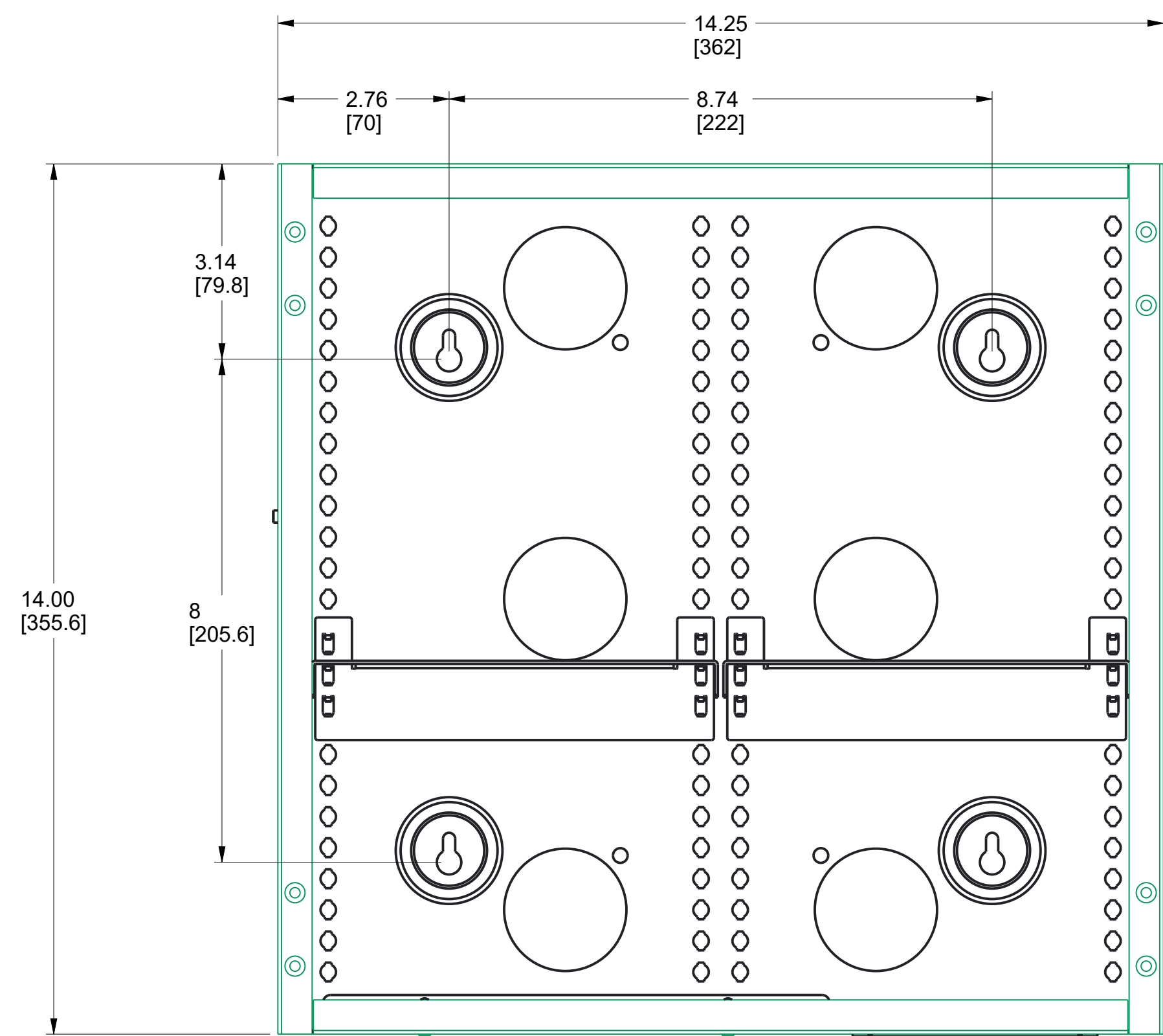
WIREFATH ONE,14IN,TOP ASSY
