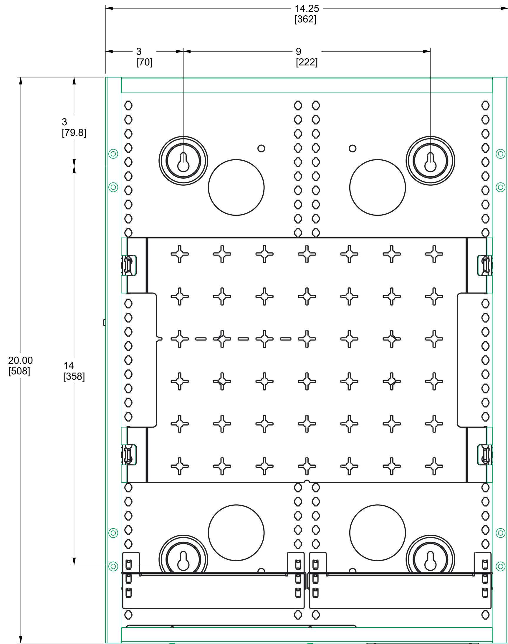
WIREFATH ONE,20IN, TOP ASSY
