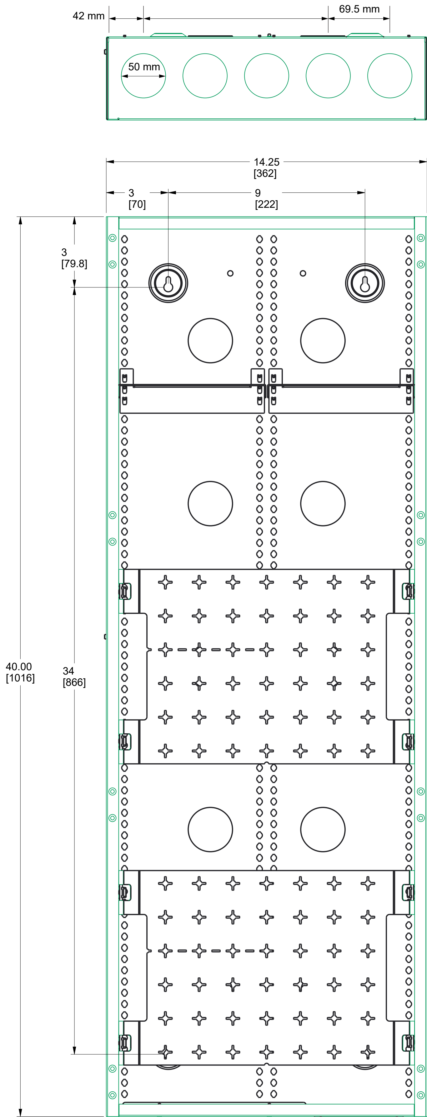
WIREFATH ONE,40IN, TOP ASSY
