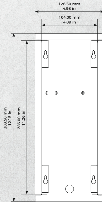
Mounting housing
